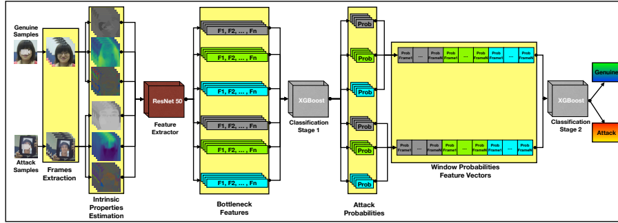
Fig. 1. Overview of the proposed method. Each video sample is split into frames and from each frame, intrinsic image properties are calculated. Then, using a ResNet50, proposed method extracts bottleneck features, which are classified by an XGBoost according probability to be an attack. Probabilities of different intrinsic properties are then combined, by using a window of N frames, where N is the small number of frames in a video of evaluated datasets, into a final feature vector which is classified according it average probability of all frames.
